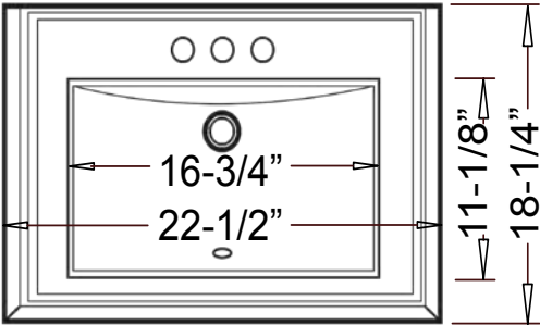
Product Diagram
